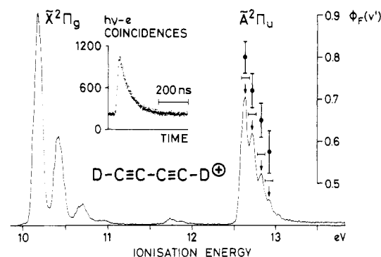
Figure 9. Photoelectron-photon coincidence curve (inset) for the \tilde{A}^2\Pi_u 0^0 level of dideuteriodiacetylene cation accumulated in about a day. Above the He I \alpha photoelectron spectrum are plotted the determined fluorescence quantum yields at the selected internal energies.
